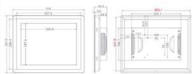
DRAWING PANEL 12.0"
