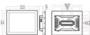
DRAWING PANEL 12,1"
